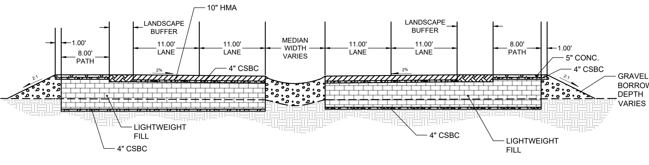
LIGHTWEIGHT FILL SECTION NTS
