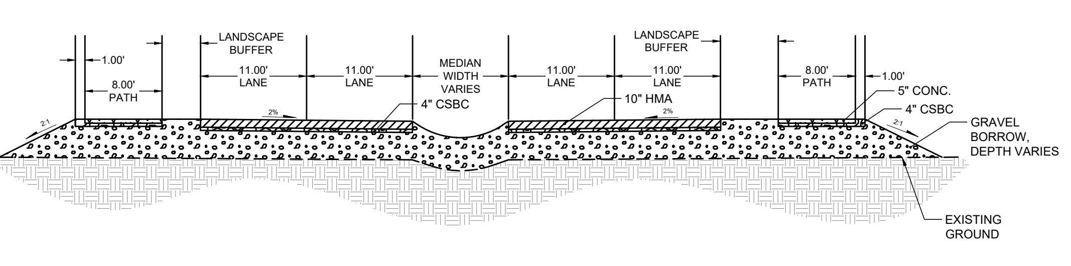
OVER-FILL SECTION NTS
