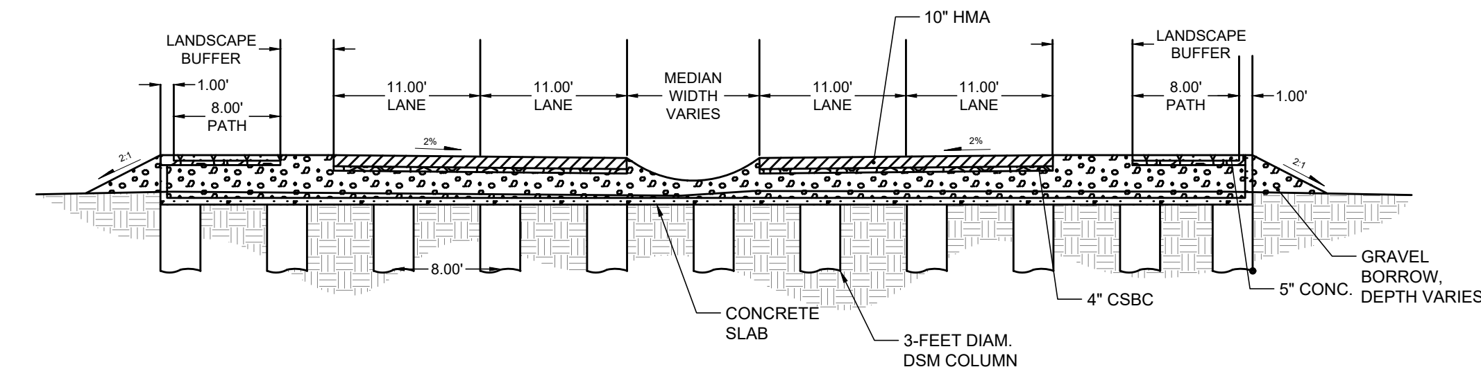
GROUND IMPROVEMENT SECTION NTS
