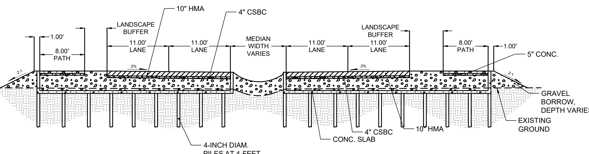
PIN-PILE SUPPORTED SLAB SECTION NTS
